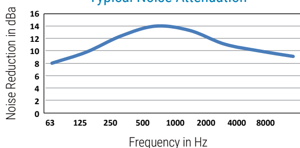
Typical Noise Attenuation
